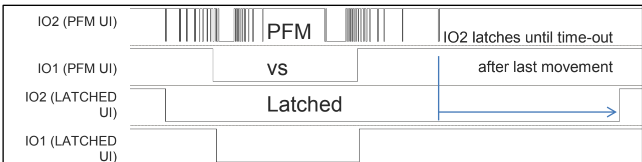
Figure 3.4 PFM movement output (TOP) compared with latched movement output (BOTTOM). Movement output is forced by first movement
