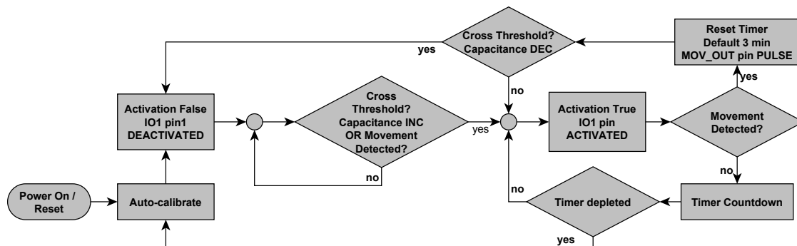
Figure 1.1 Flow diagram of the typical IQS211 movement based user interface
