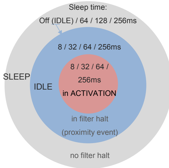
Figure 1.11 Low power mode description from outside (no interaction), to inside (full interaction)
