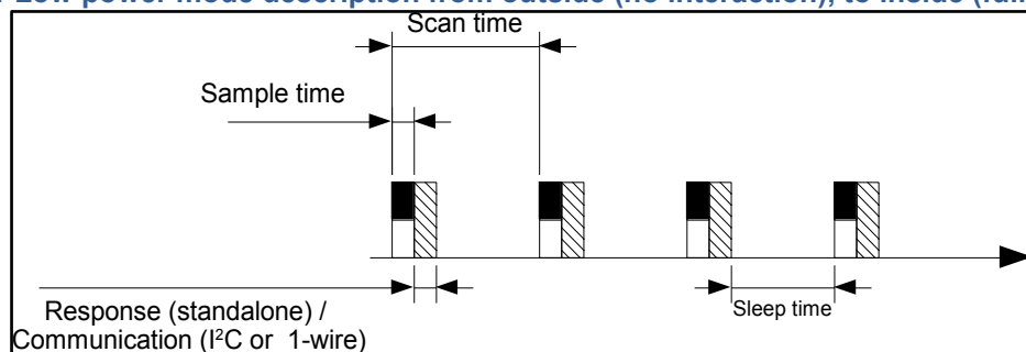
Figure 1.12 Sample-, scan-, sleep- and communication time diagram
