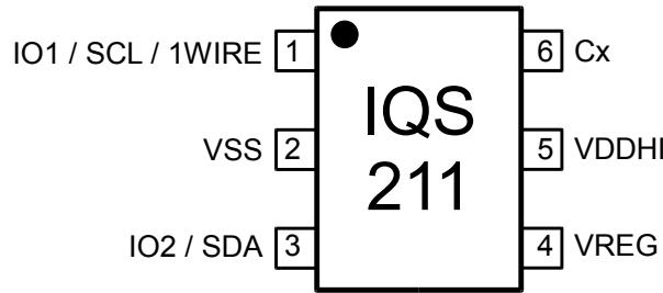
Figure 2.1 IQS211 pin-out (TSOT23-6 package)
