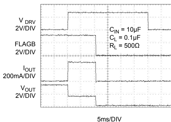
Figure 14. T_{\text{BLANK}} Response
