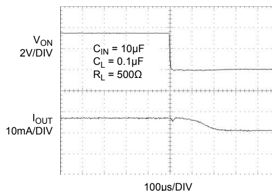
Figure 16. T_{\text{OFF}} Response
