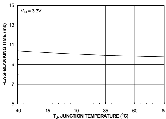
Figure 13. T_{\text{BLANK}} vs. Temperature
