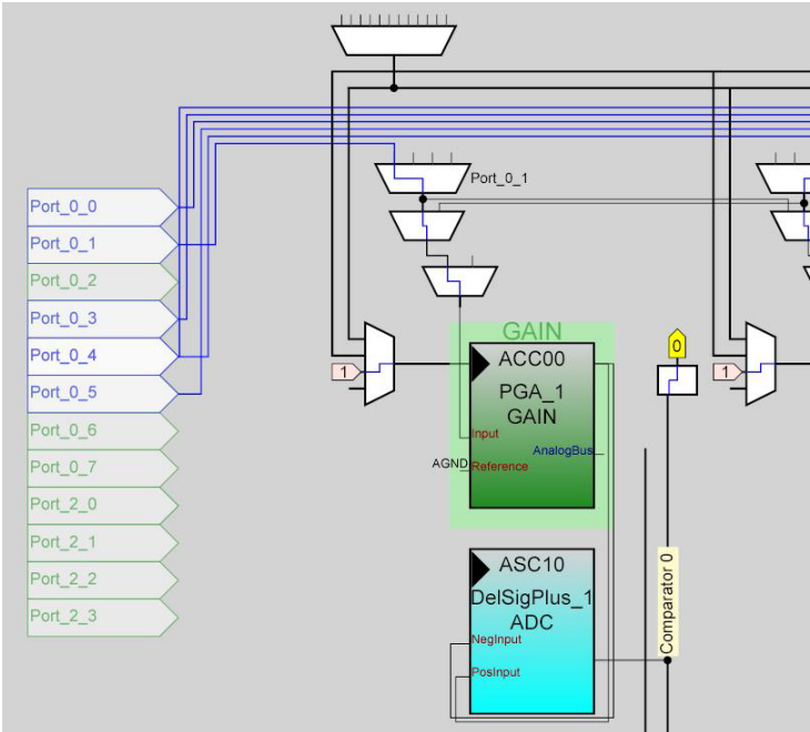
Figure 3-16. Place PGA in ACC00
