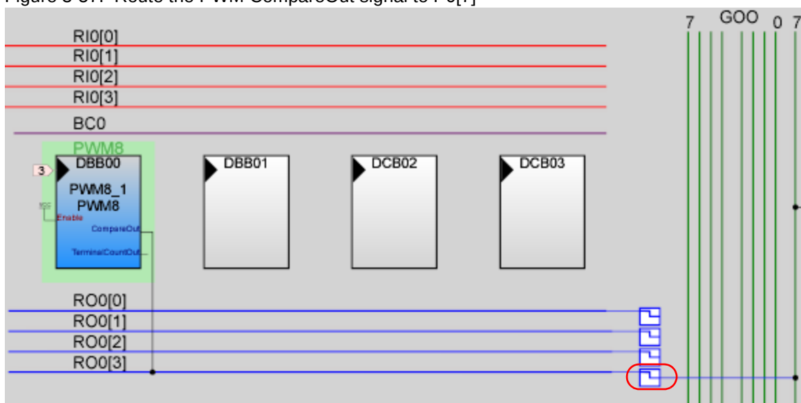
Figure 3-57. Route the PWM CompareOut signal to P0[7]
