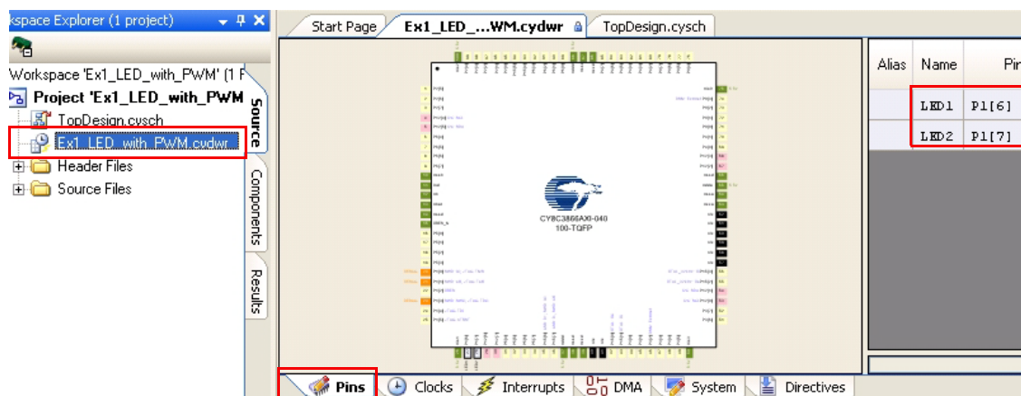
Figure 3-100. Pin Assignments
