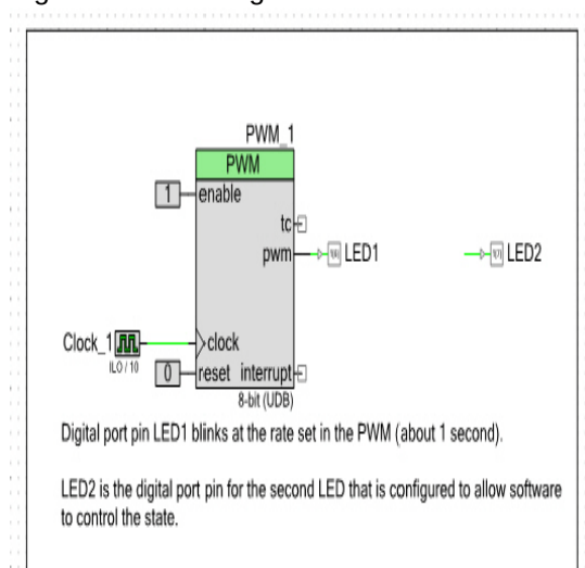
Figure 3-49. Configure Global Resources
