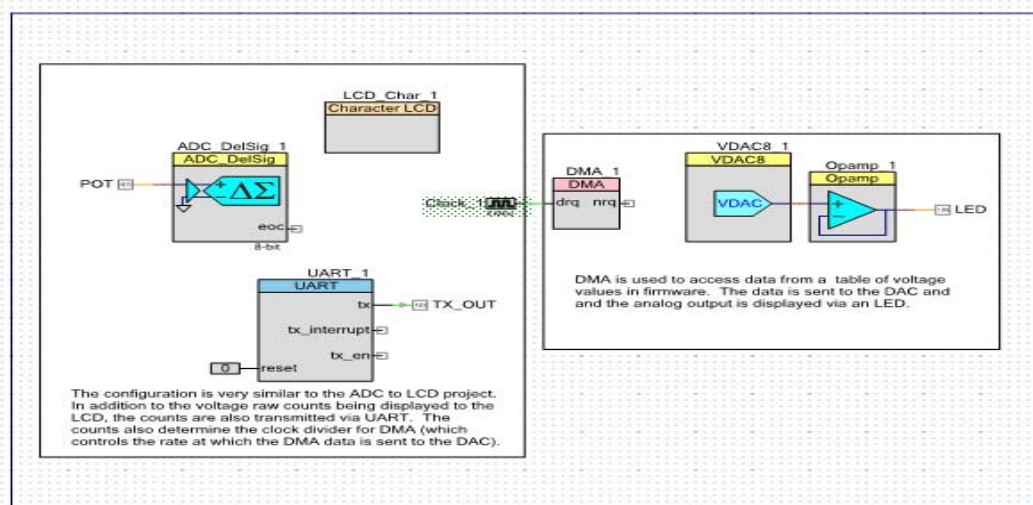
Figure 3-119. Connected Components
