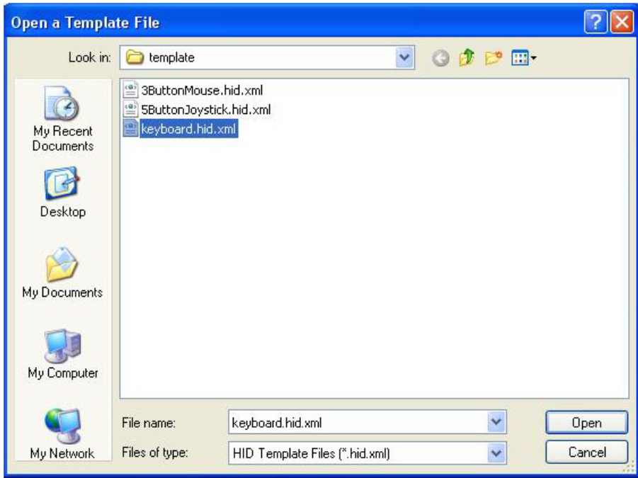
Figure 3-123. USB Template
