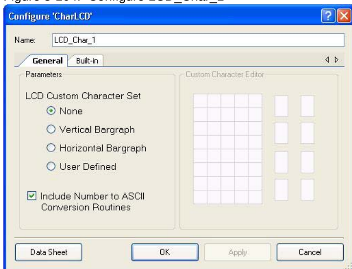
Figure 3-104. Configure LCD_Char_1
