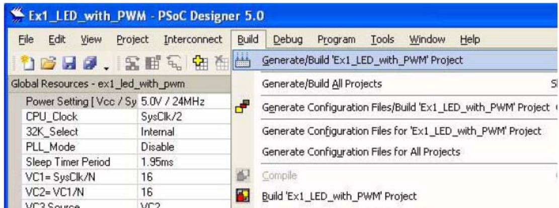
Figure 2-2. Build Project
