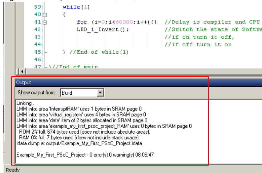
Figure 2-8. Output Window
