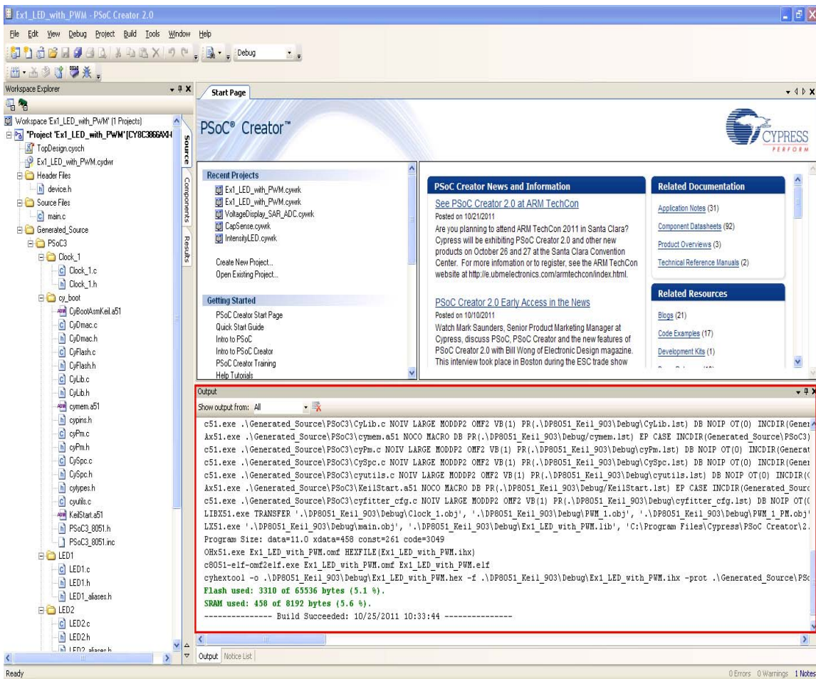
Figure 2-15. Output Window
