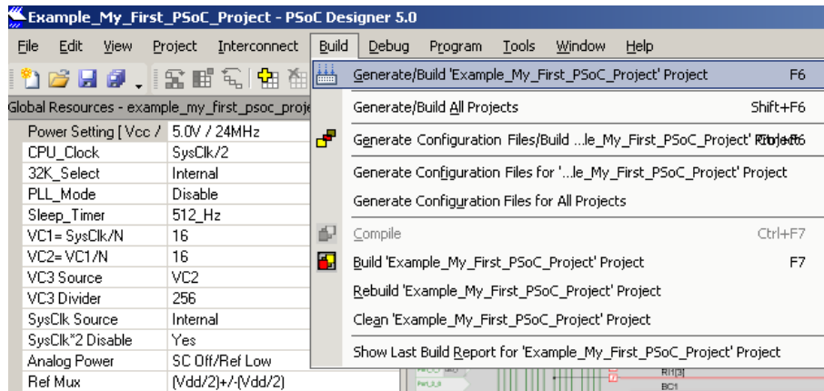
Figure 2-7. Build Project
