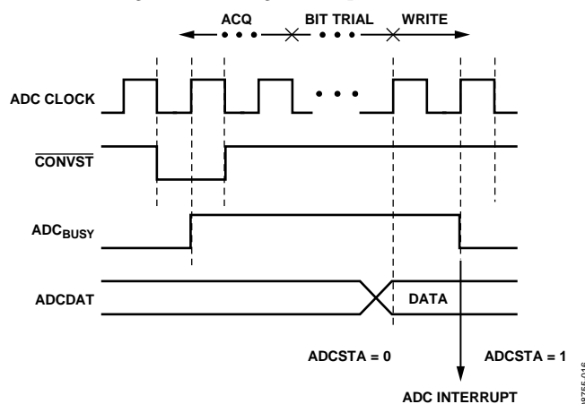
Figure 16. ADC Timing
