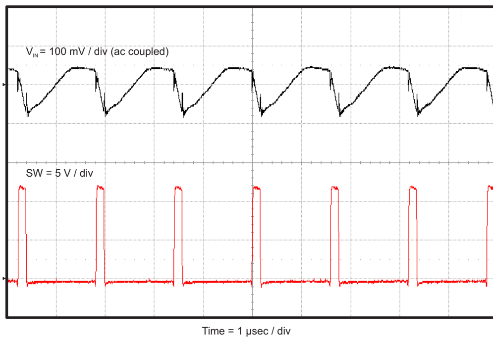
Figure 9. TPS562200EVM-601 Input Voltage Ripple, I_{OUT} = 2 A
