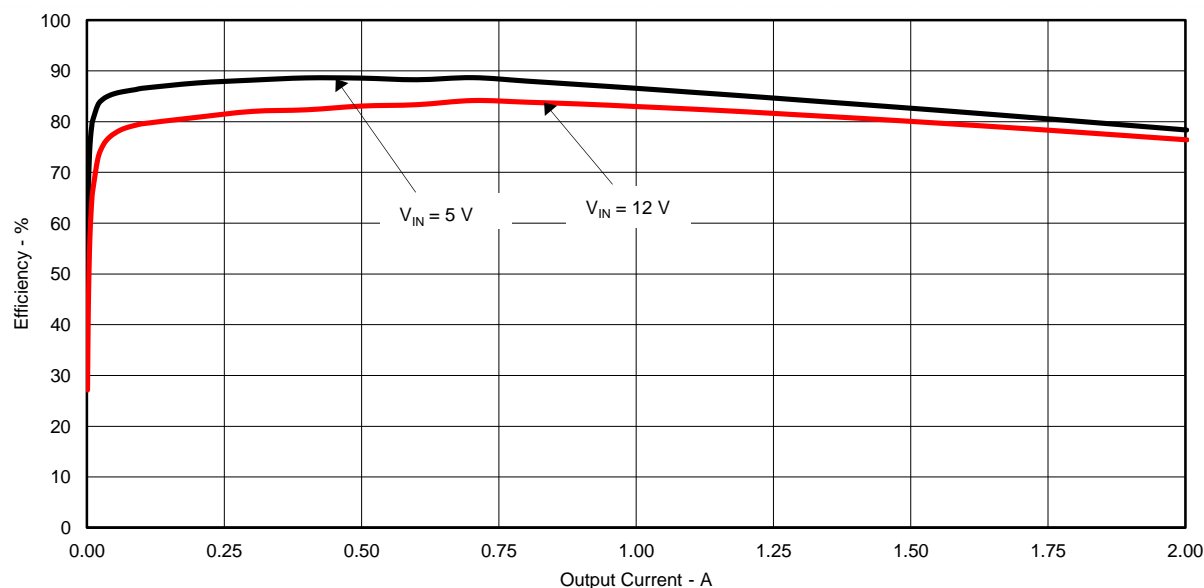
Figure 1. TPS562200EVM-601 Efficiency
