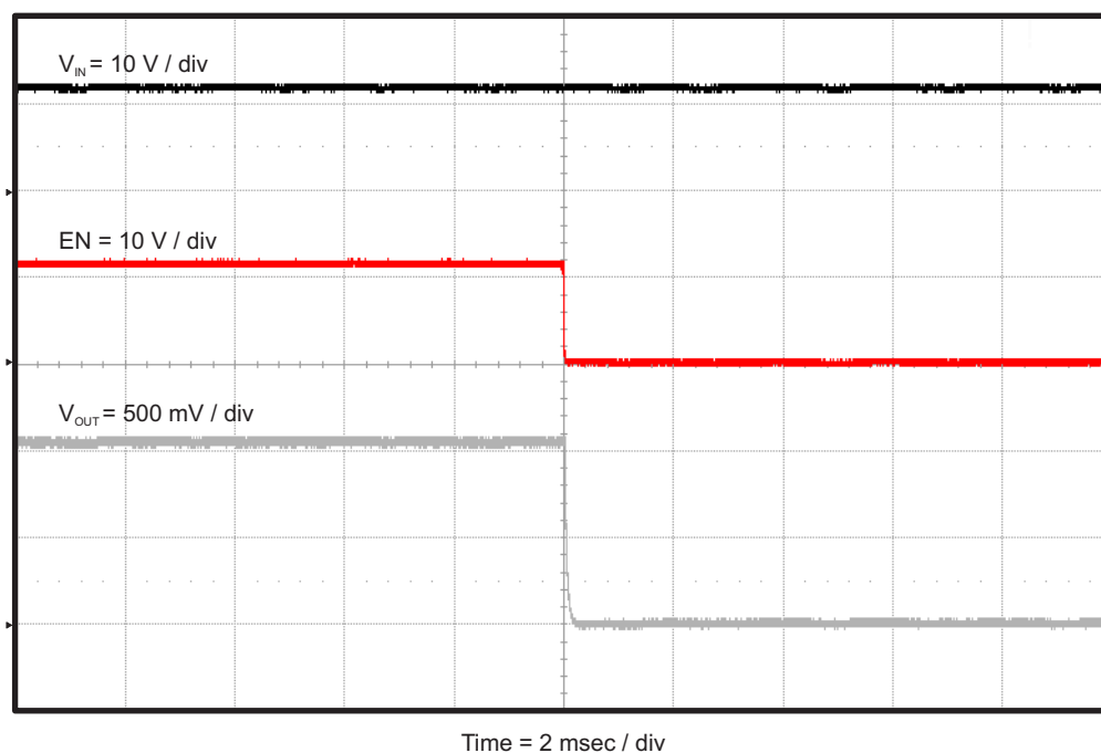
Figure 13. TPS562200EVM-601 Shut-Down Relative to EN
