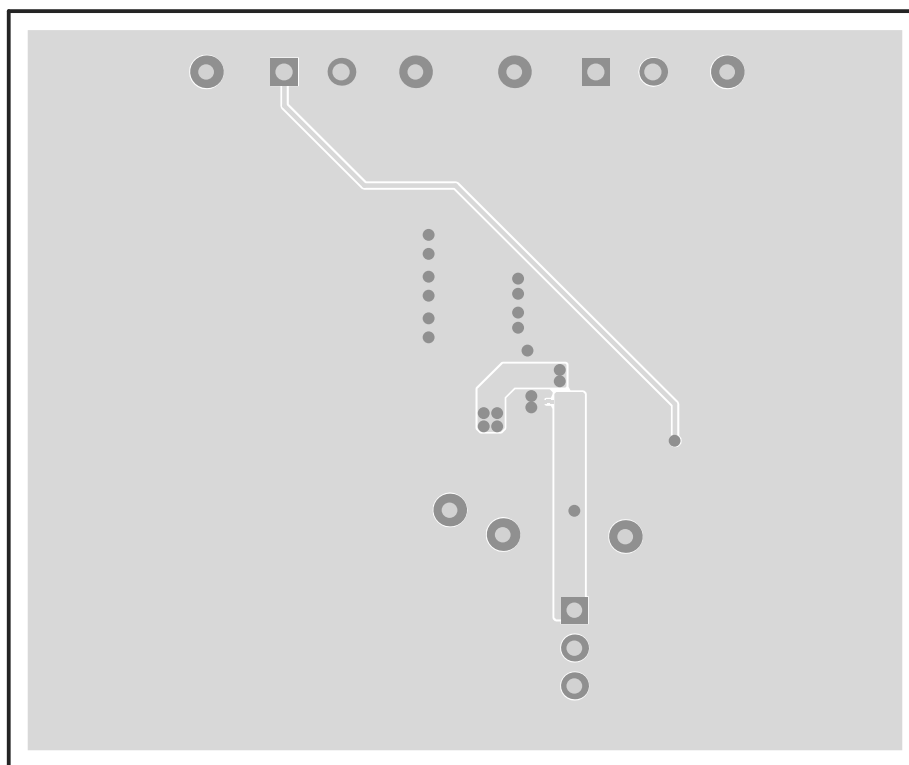
Figure 15. Bottom Layer
