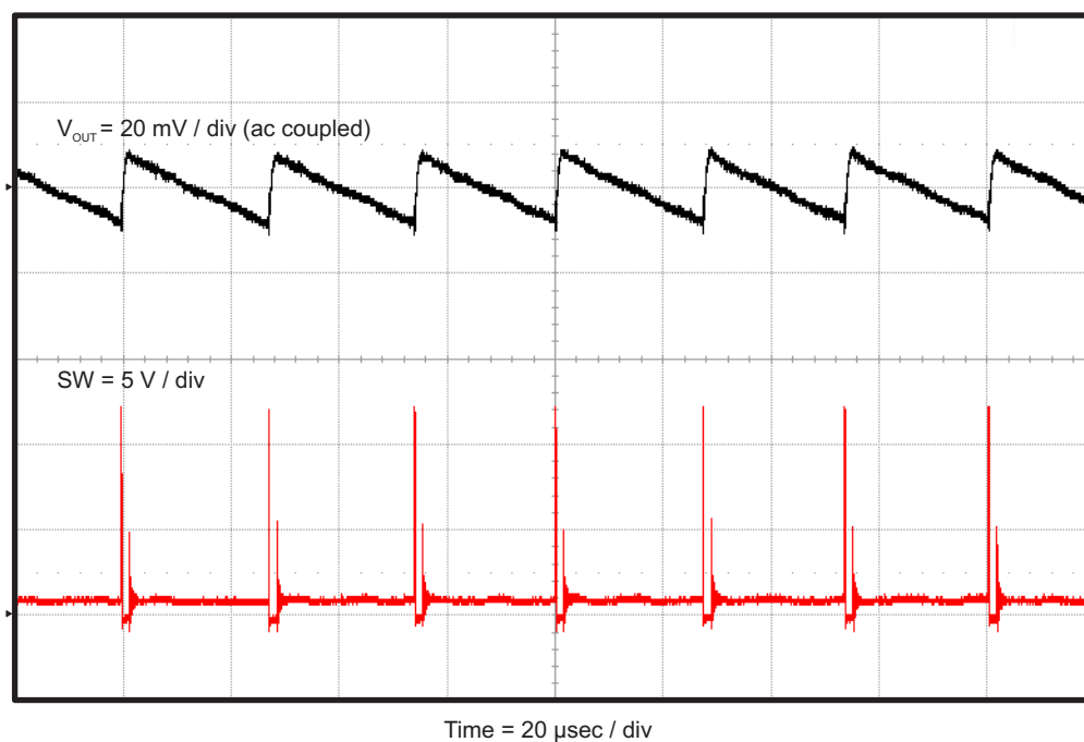
Figure 8. TPS562200EVM-601 Output Voltage Ripple, I_{OUT} = 10 mA
