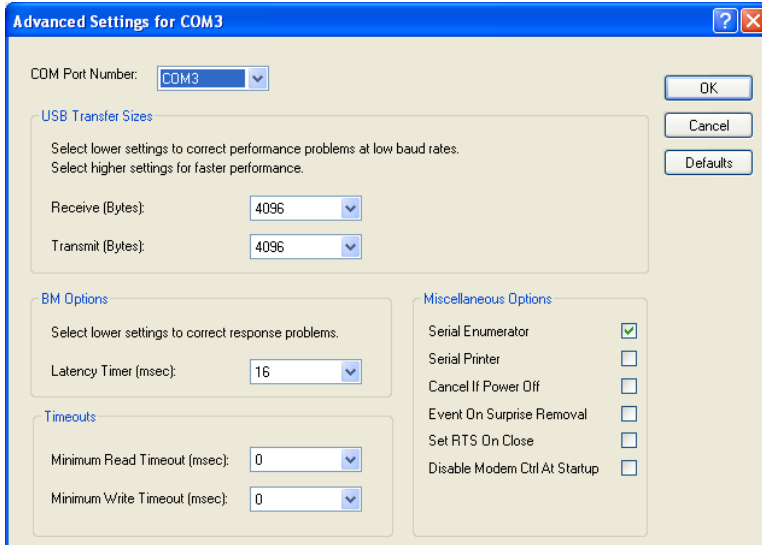
Figure 2.10 - Advanced Options
