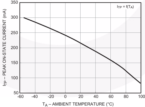
Figure 12. Current Reduction
