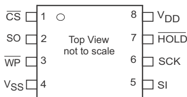
Figure 2. 8-pin TDFN pinout
