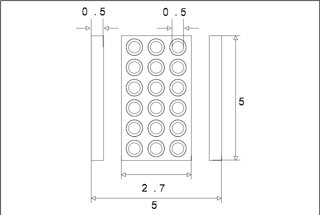
Figure 15. Recommended footprint
