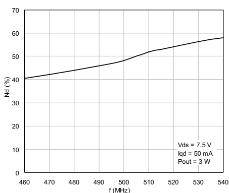
Figure 11. Efficiency vs frequency
