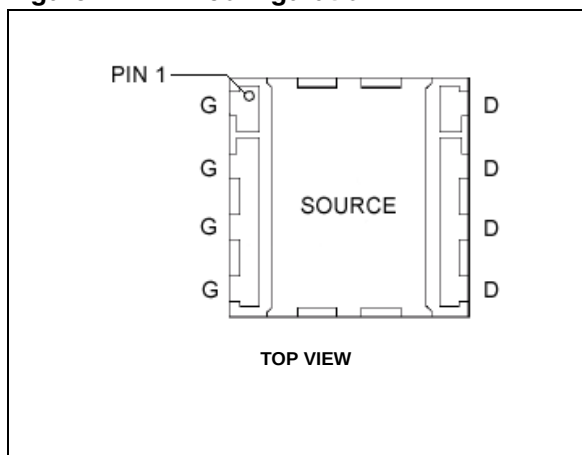
Figure 1. Pin configuration
