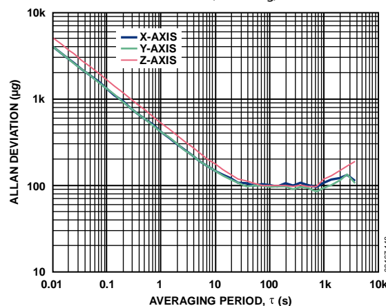
Figure 55. Allan Deviation
