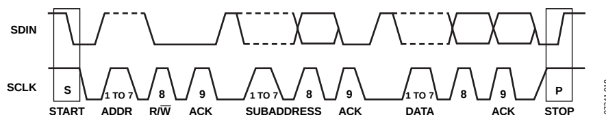
Figure 28. 2-Wire I 2 C Generalized Clocking Diagram
