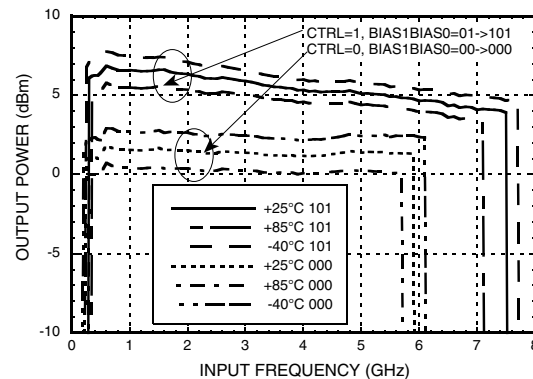
Output Power vs. Temperature Divide-by-4
