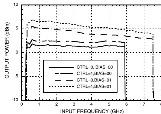
Pout Divide-by-4 vs. CTRL & BIAS
