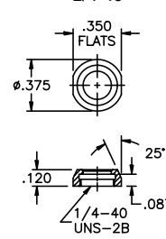
PANEL DRESS NUT A168P1 Blind thread, Nickel plated brass 1/4-40
