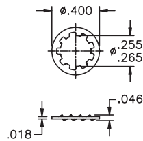
PUSHBUTTON CAP A212
