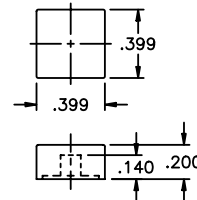
PUSHBUTTON CAP A235
