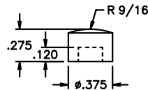
PUSHBUTTON CAP A212
