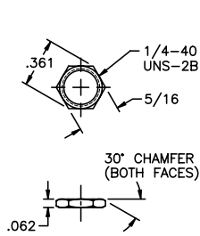
HEX NUT A112 Nickel plated brass 1/4-40
