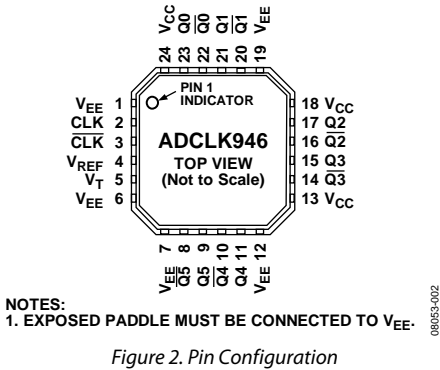
Figure 2. Pin Configuration
