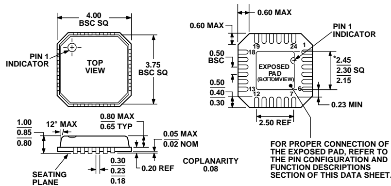
Figure 23. 24-Lead Lead Frame Chip Scale Package [LFCSP_VQ] 4 mm x 4 mm Body, Very Thin Quad CP-24-2 Dimensions shown in millimeters
