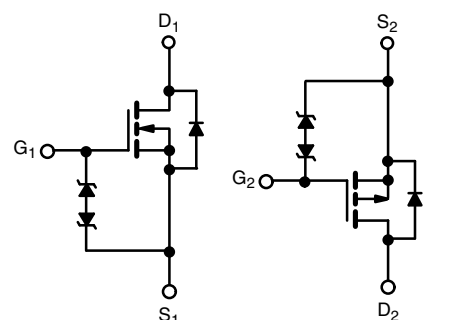
N-Channel MOSFET
