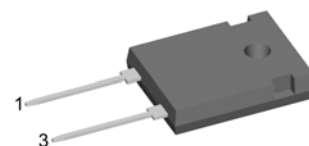
Backside: cathode
