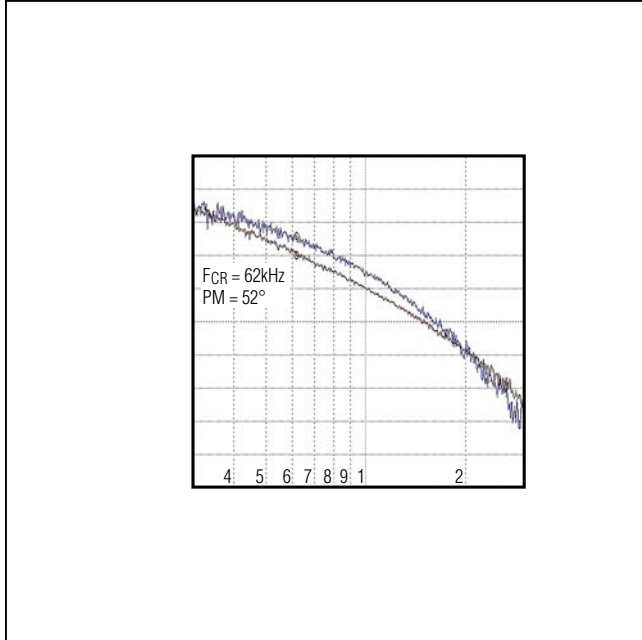
Figure 3. MAX17501G Full-Load Bode Plot ( V_{IN} = 24V )
