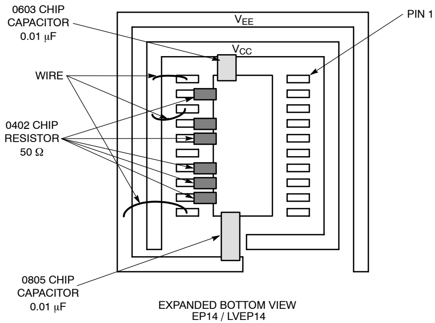
Figure 6. Configuration 1
