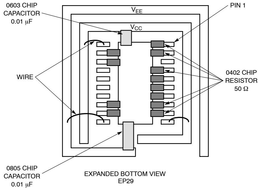
Figure 8. Configuration 3
