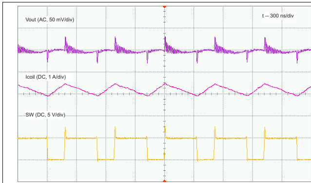
Figure 19. PWM Operation ( V_{OUT} = 5\text{ V} , I_{OUT} = 2\text{ A} )
