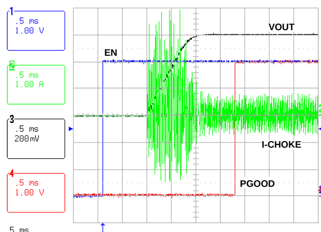
FIGURE 4. OUTPUT CAPACITOR IN-RUSH CURRENT: 50Ω LOAD, FCCM = HIGH, 1V VOUT-PREBIAS
