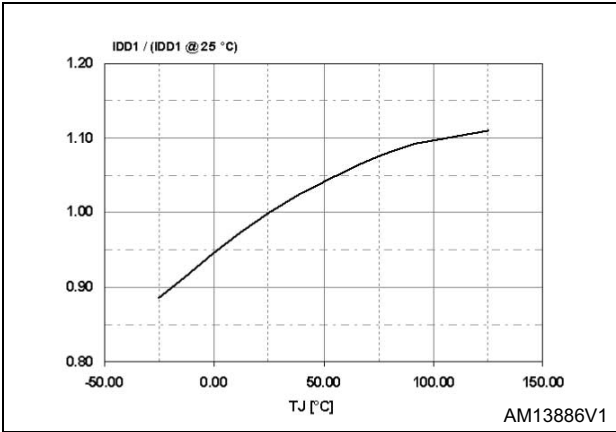
Figure 10. I_{DD1} vs. T_J
