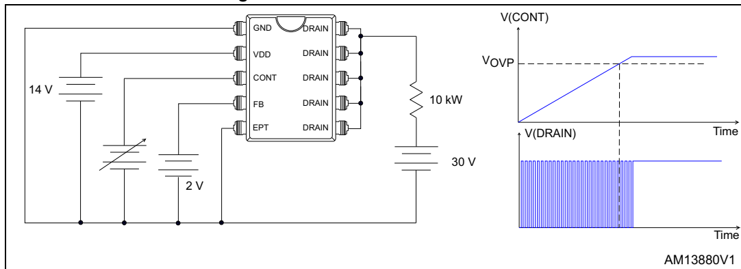
Figure 5. OVP threshold test circuit
