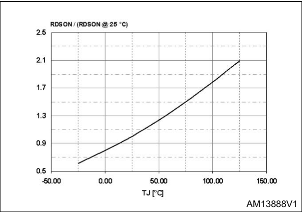
Figure 11. Main FET R_{DS(on)} vs. T_J
