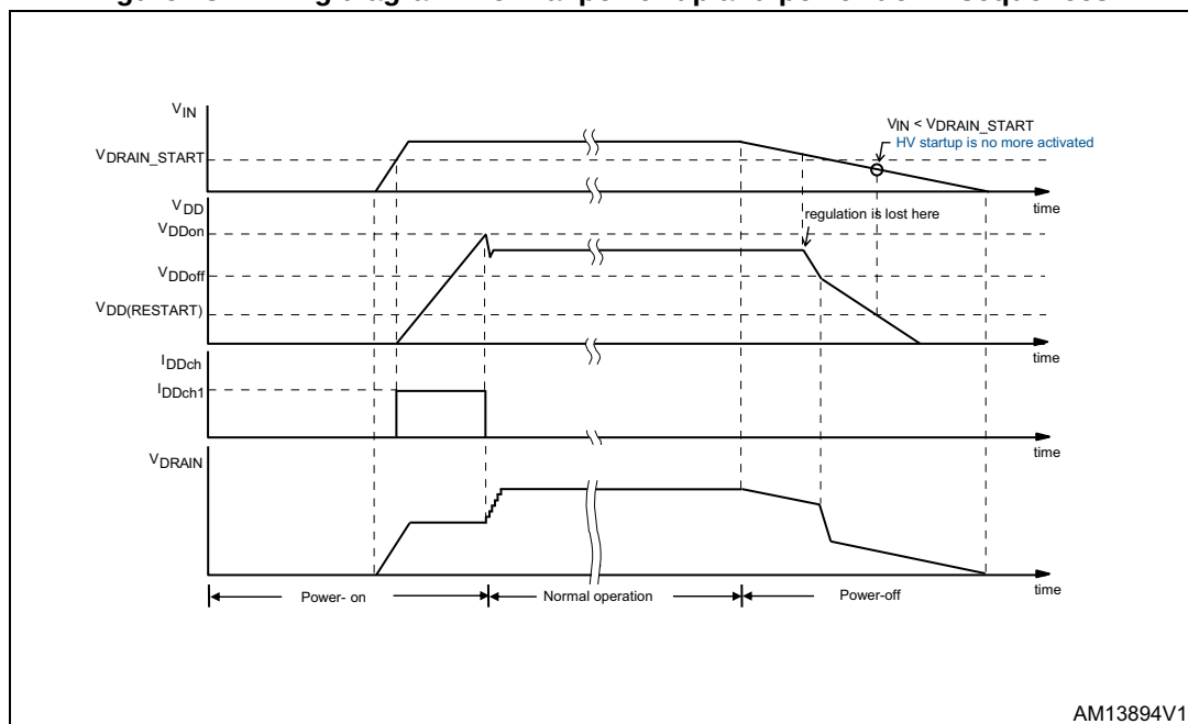
Figure 18. Timing diagram: normal power-up and power-down sequences
