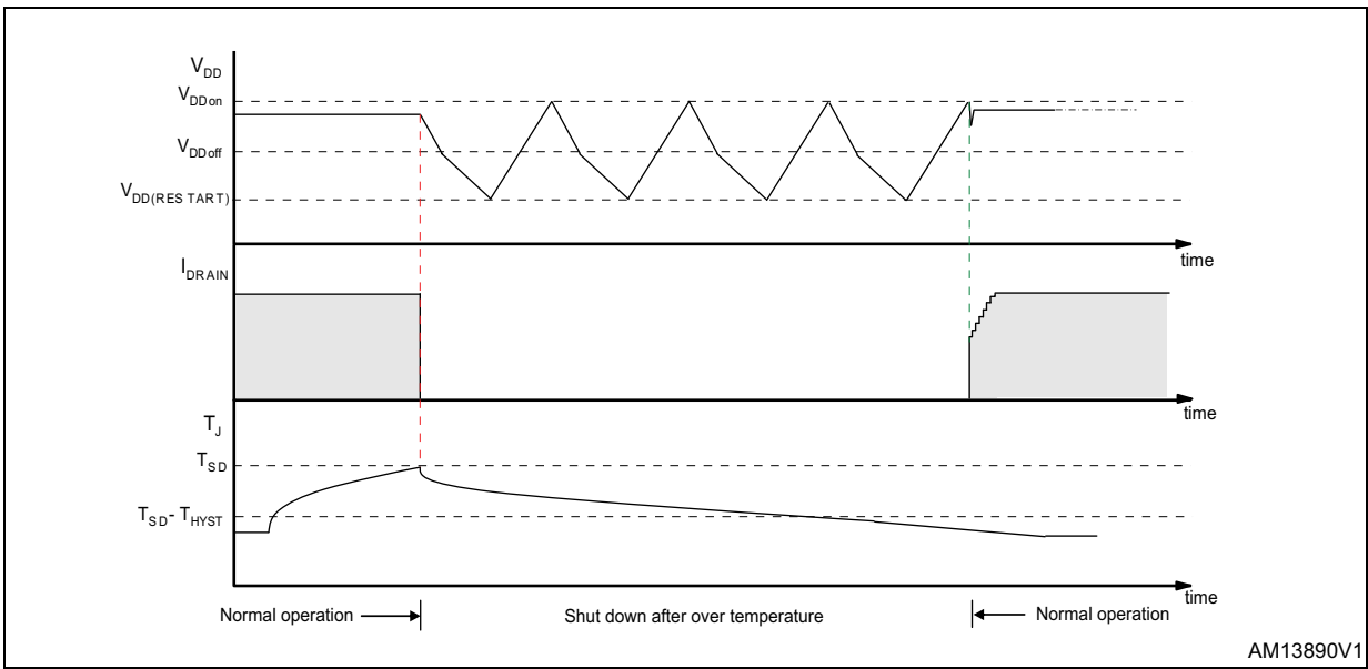
Figure 14. Thermal shutdown
