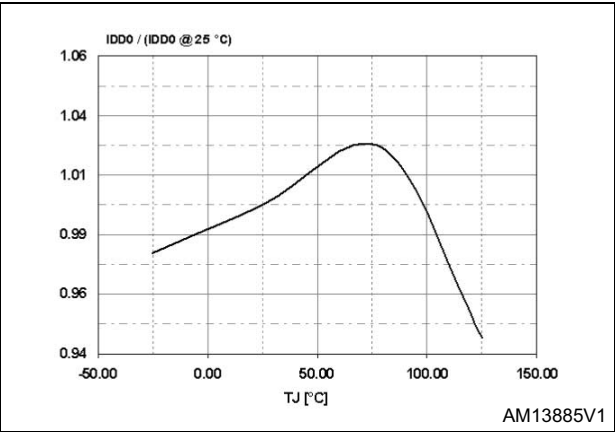
Figure 9. I_{DD0} vs. T_J
