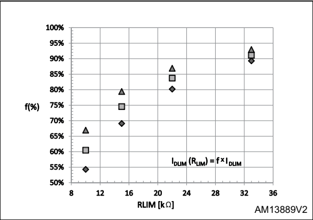
Figure 13. I_{Dlim} vs. R_{LIM}
