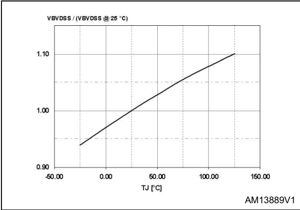
Figure 12. Main FET V_{BVDSS} vs. T_J
