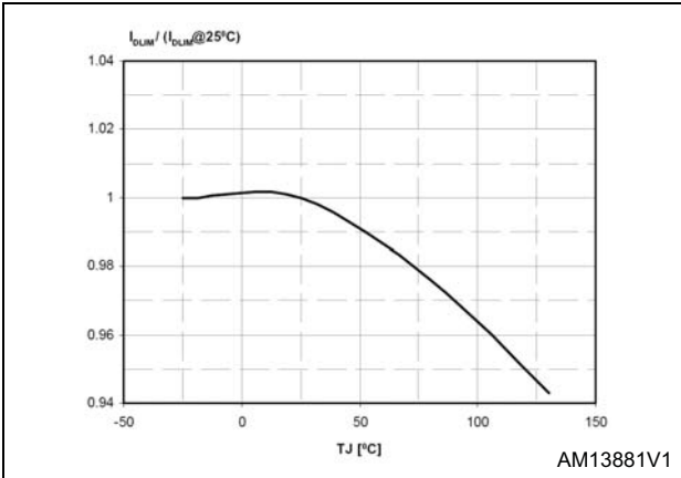
Figure 6. I_{Dlim} vs. T_J
