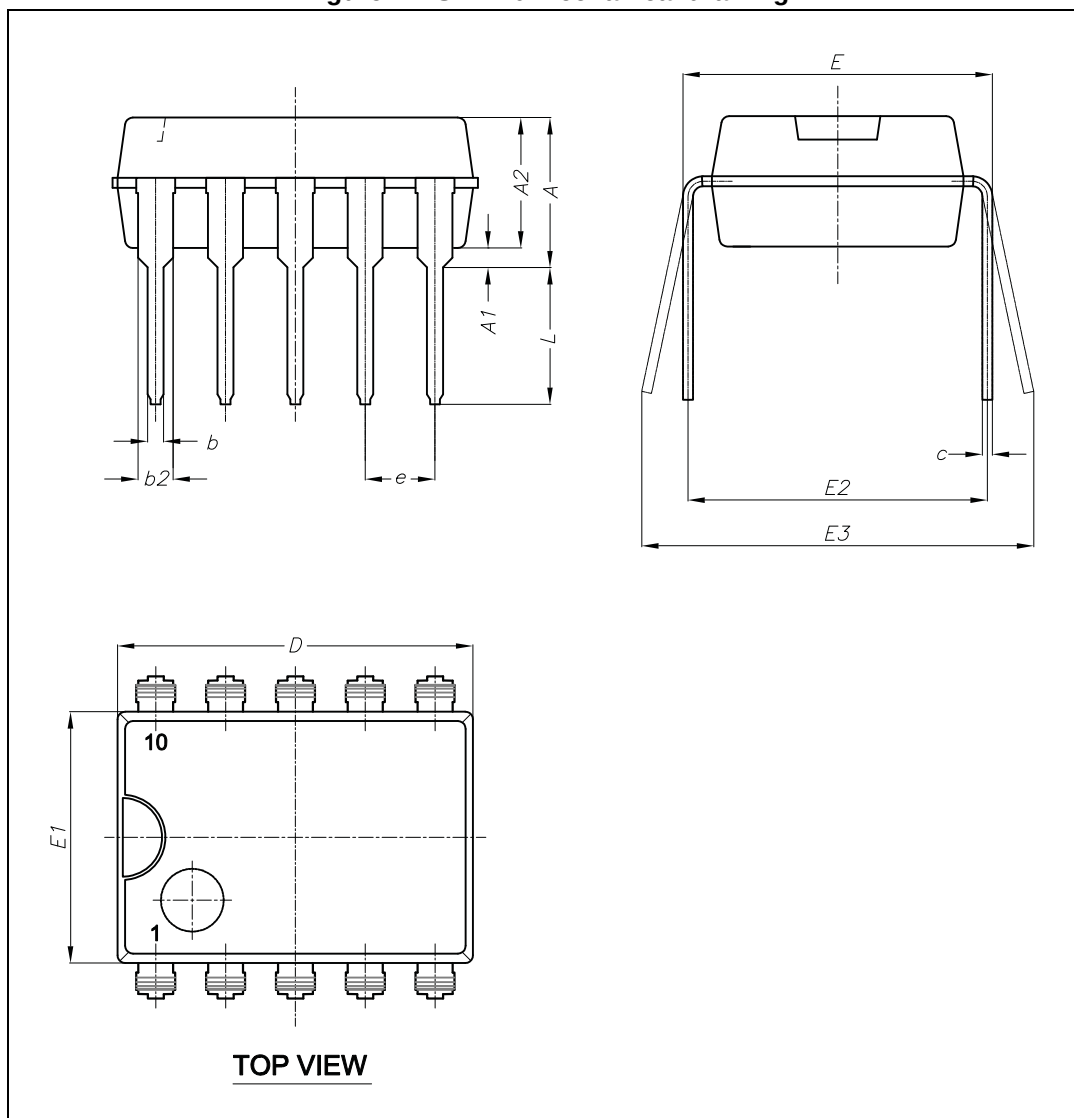
Figure 27. SDIP10 mechanical drawing
