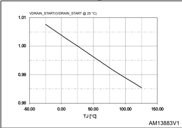
Figure 8. V_{DRAIN\_START} vs. T_J
