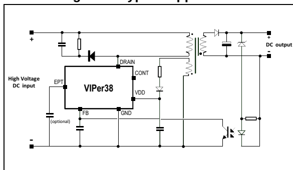
Figure 1. Typical application
