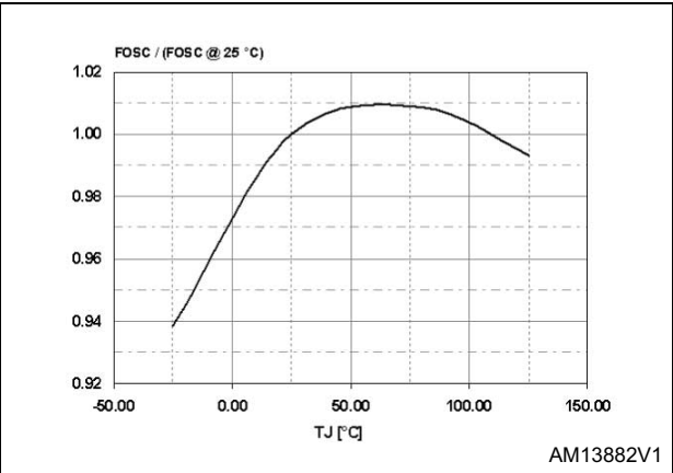
Figure 7. F_{OSC} vs. T_J
