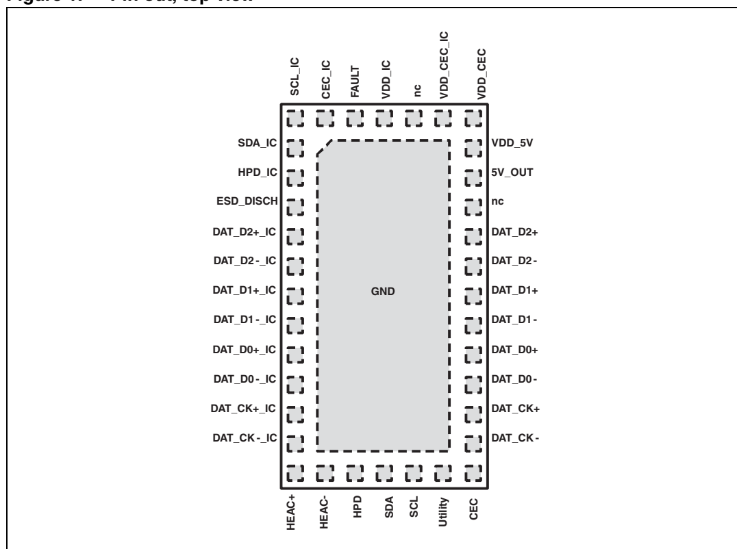
Figure 1. Pin out, top view
