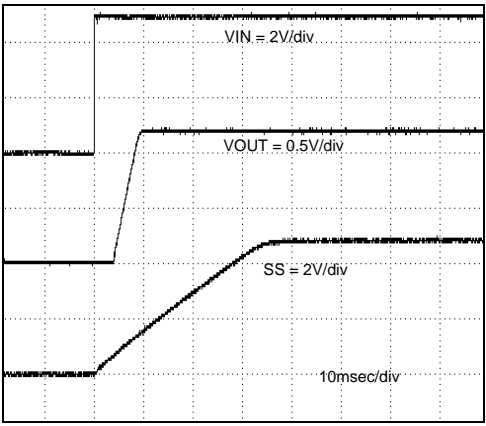
Fig.14 Soft start
