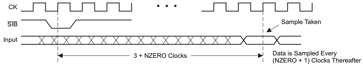
Figure 1-5. Zero-Pad Synchronization
