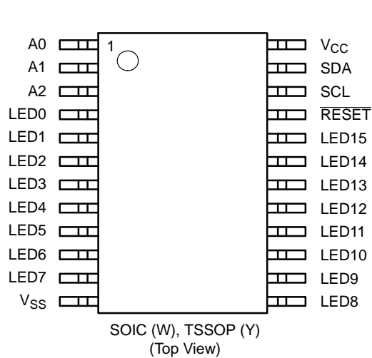
Figure 1. Pin Configurations
