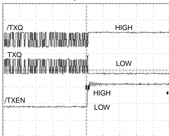
Output Disable
