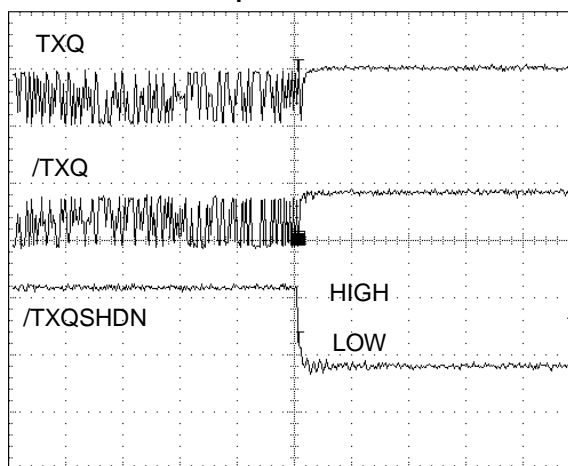
Output Shutdown
