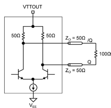
Figure 7a. CML DC-Coupled Termination
