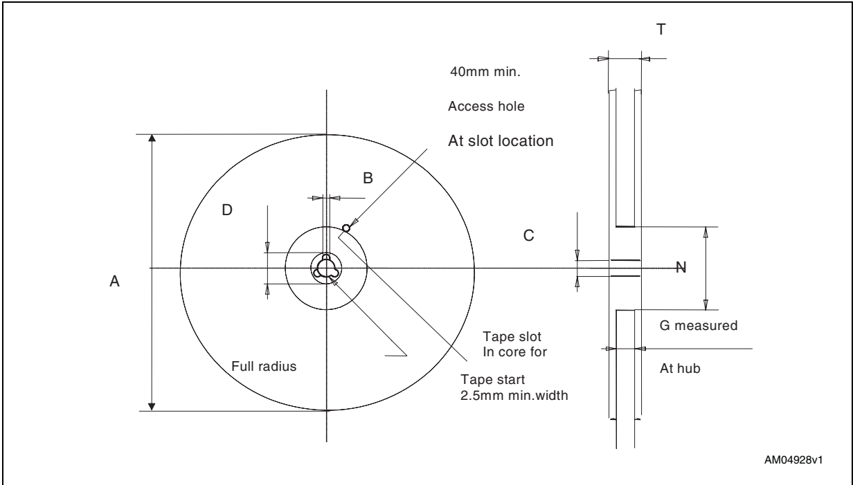
Figure 19. Reel schematic
