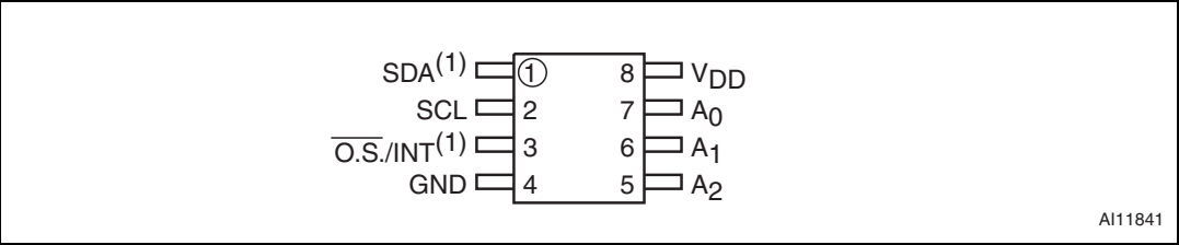
Figure 2. Connections
