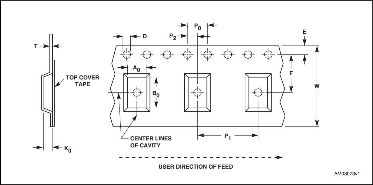
Figure 18. Carrier tape for MSOP8 (TSSOP8) package
