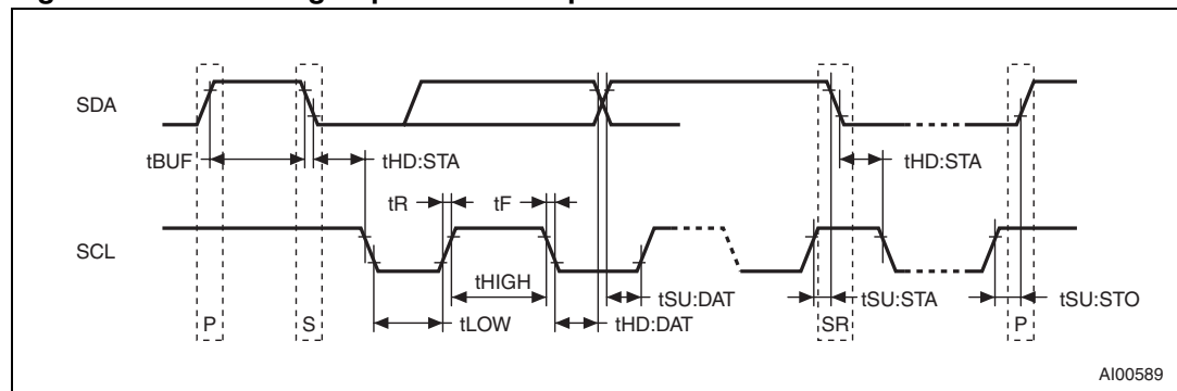
Figure 16. Bus timing requirements sequence
