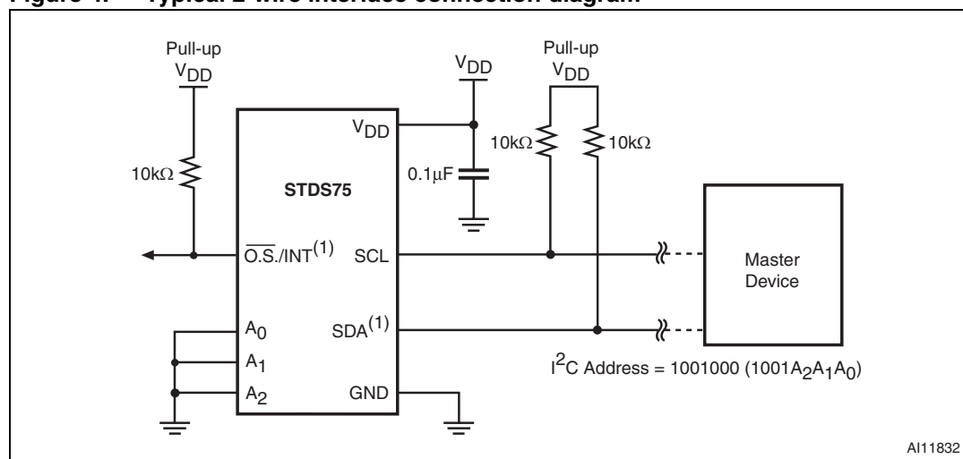
Figure 4. Typical 2-wire interface connection diagram
