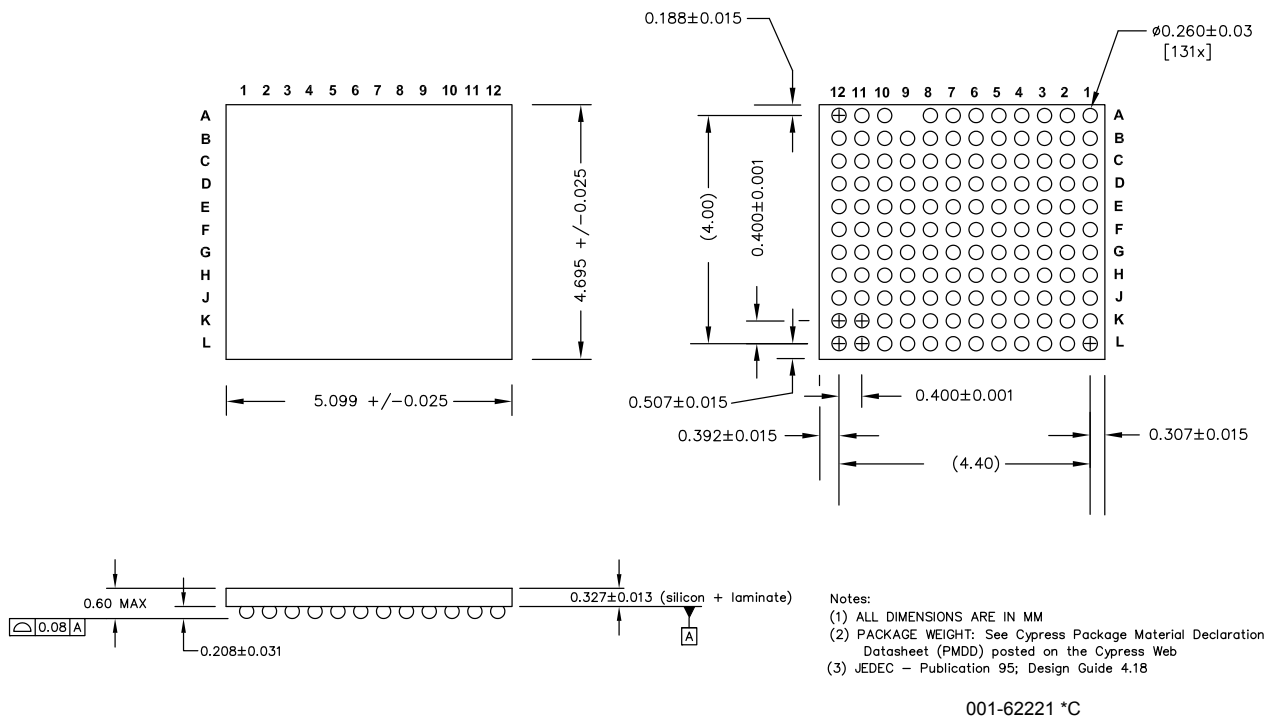
Figure 9. 131-ball WLCSP FB131/FN131 Package Outline, 001-62221
