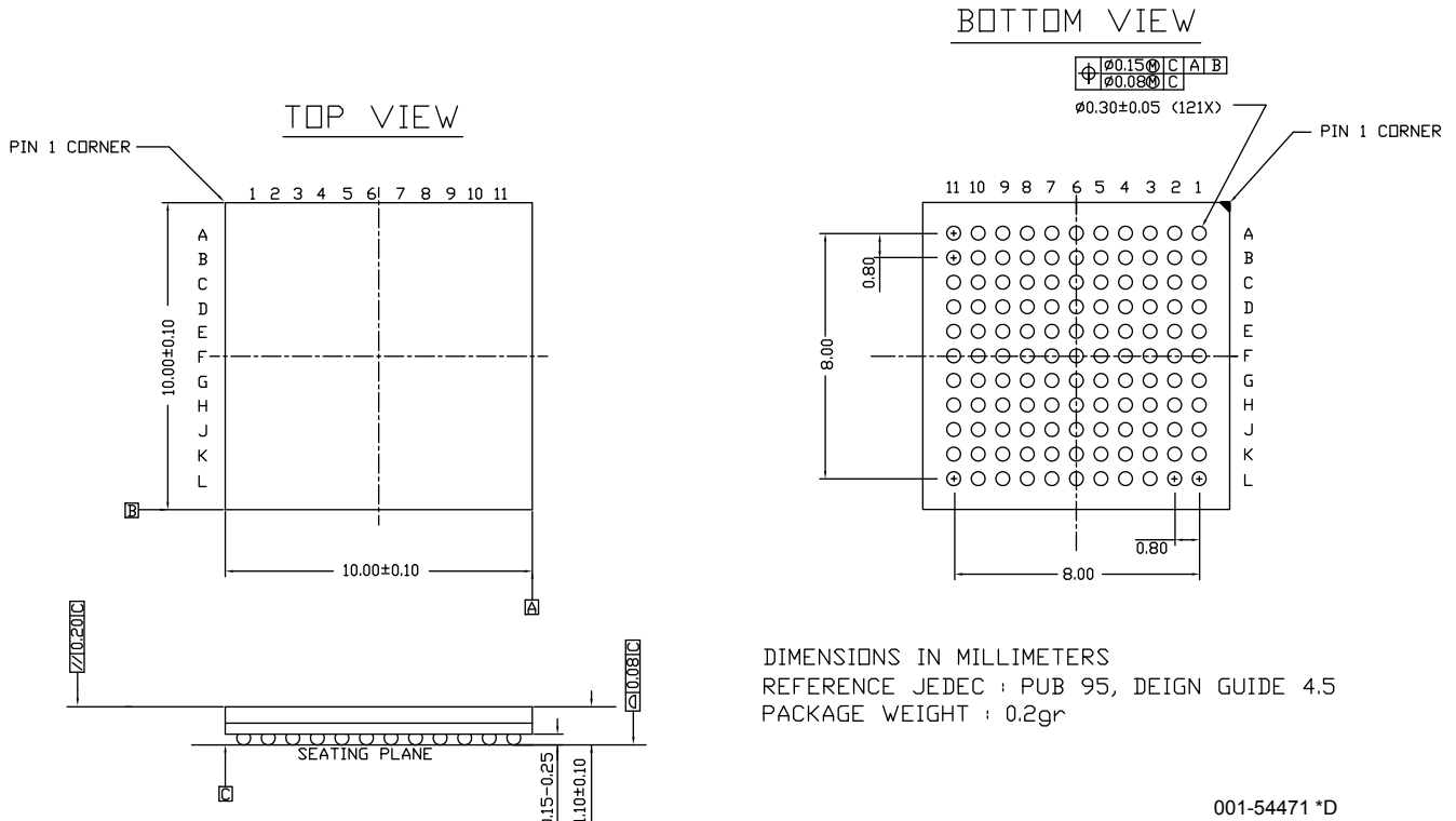
Figure 8. 121-ball FBGA (10 × 10 × 1.20 mm) Package Outline, 001-54471
