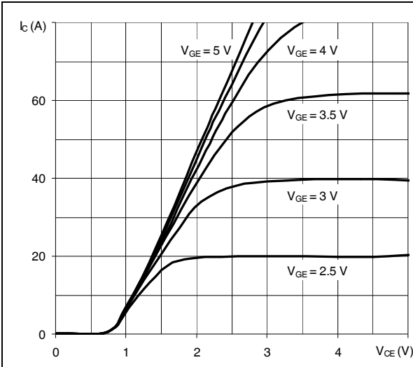
Figure 4. Output characteristics ( T_J = 25\text{ }^{\circ}\text{C} )
