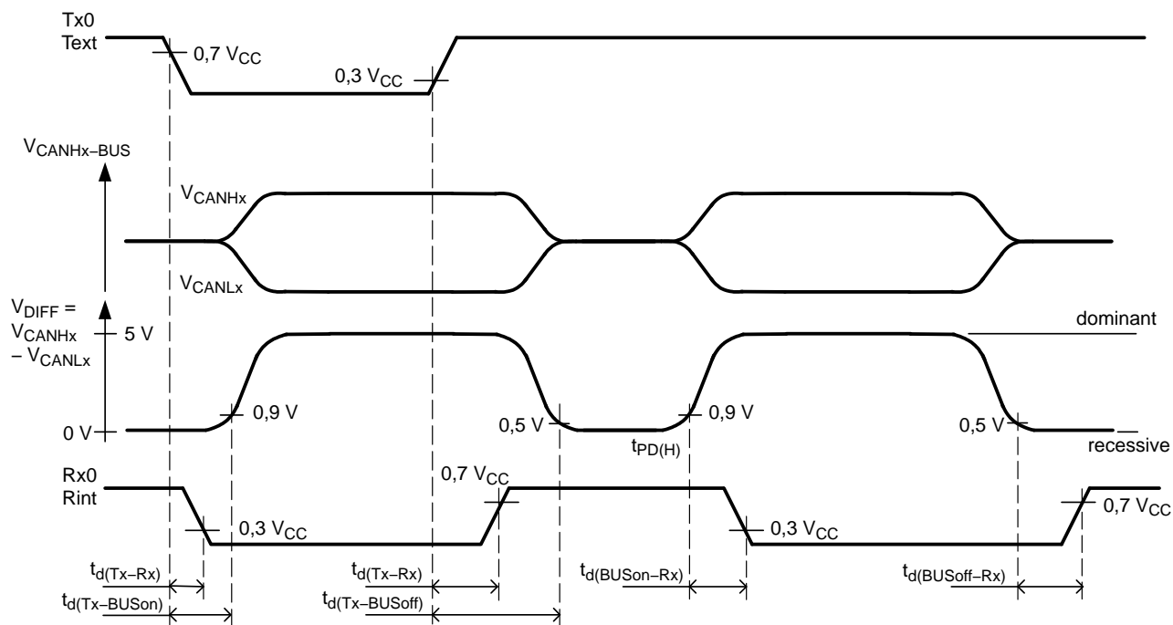
Figure 9. Timing Diagram for AC Characteristics
