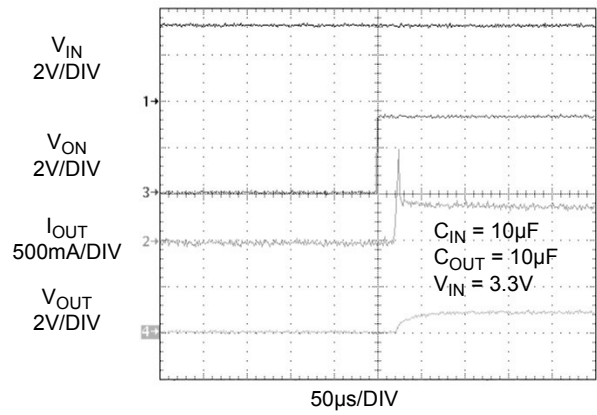
Figure 20. Current Limit Response Time (Output is loaded by 2.2Ω, C OUT = 10µF)
