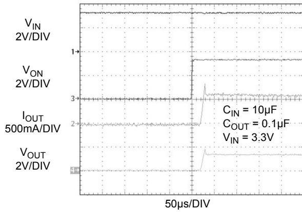
Figure 19. Current Limit Response Time (Output is loaded by 2.2Ω, C OUT = 0.1µF)
