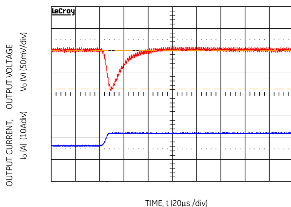
Figure 34. Transient Response to Dynamic Load Change from 50% to 100% at 12Vin, C_{out}=5\times 47\mu\text{F} , C_{Tune}=1500\text{pF} & R_{Tune}=330\Omega
