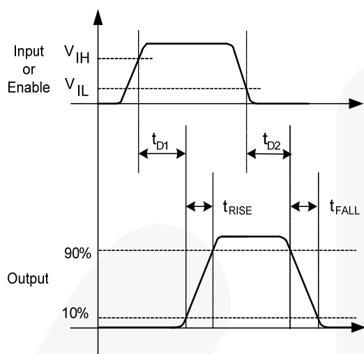
Figure 8. Non-Inverting
