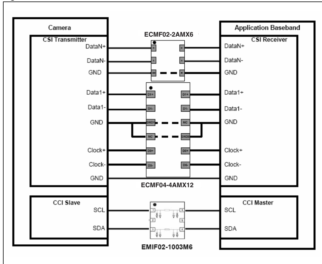
Figure 15. MIPI D-PHY
