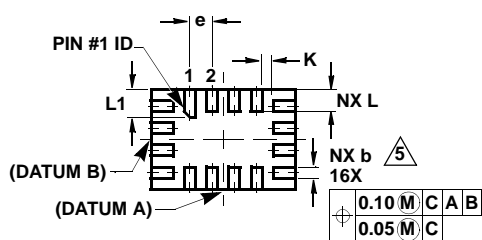
BOTTOM VIEW
