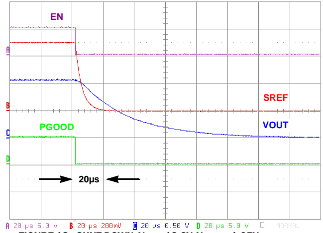
FIGURE 18. SHUT-DOWN, V_{IN} = 12.6V , V_{OUT} = 1.05V , LOAD = 50m\Omega
