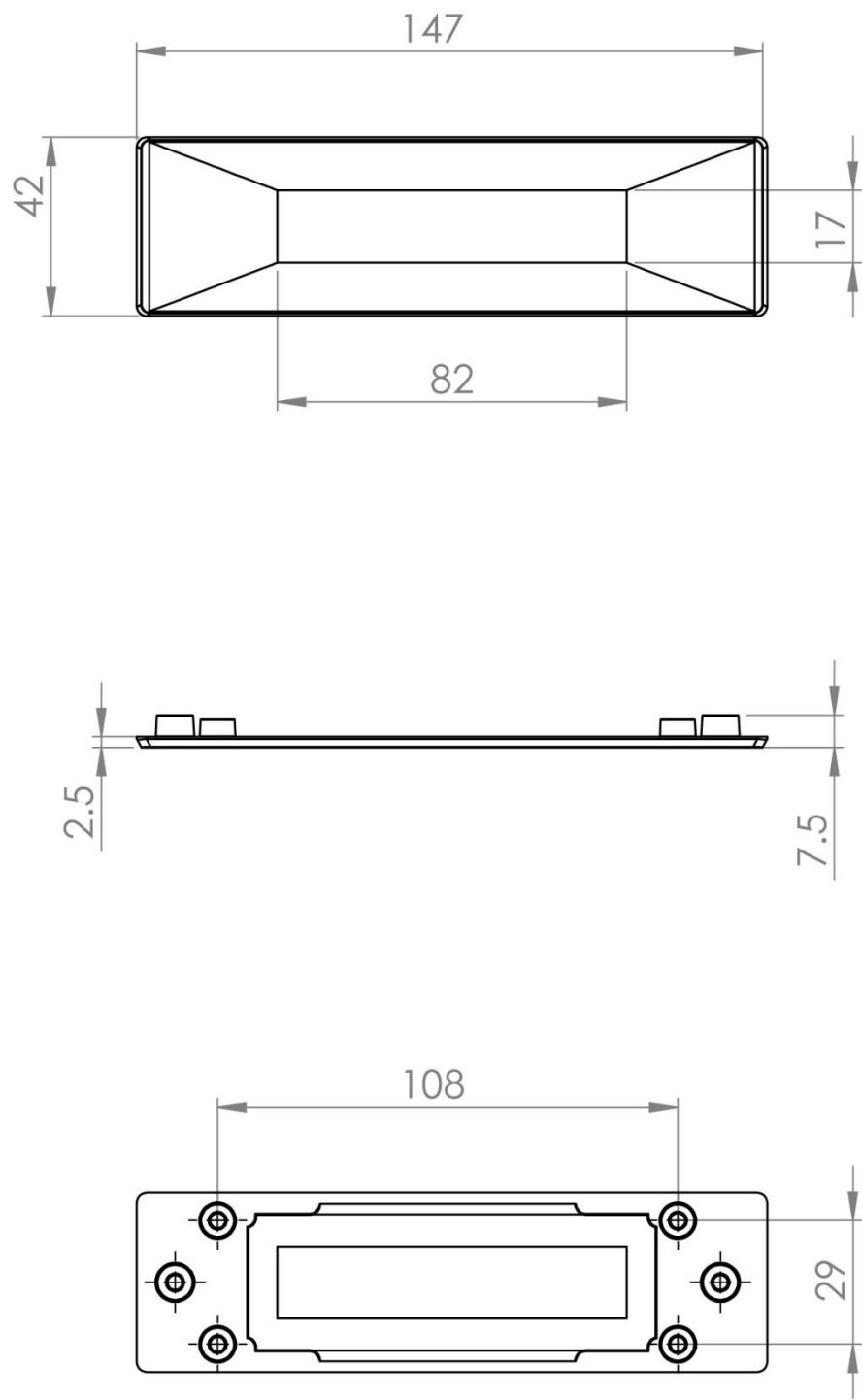
Figure 3: Bez-202C-V1 Dimensions
