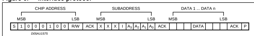
Figure 6. Interface protocol
