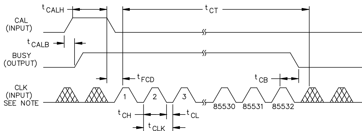
CALIBRATION TIMING
