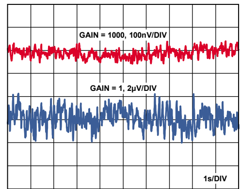
Figure 27. 0.1 Hz to 10 Hz RTI Voltage Noise ( G = 1 , G = 1000 )
