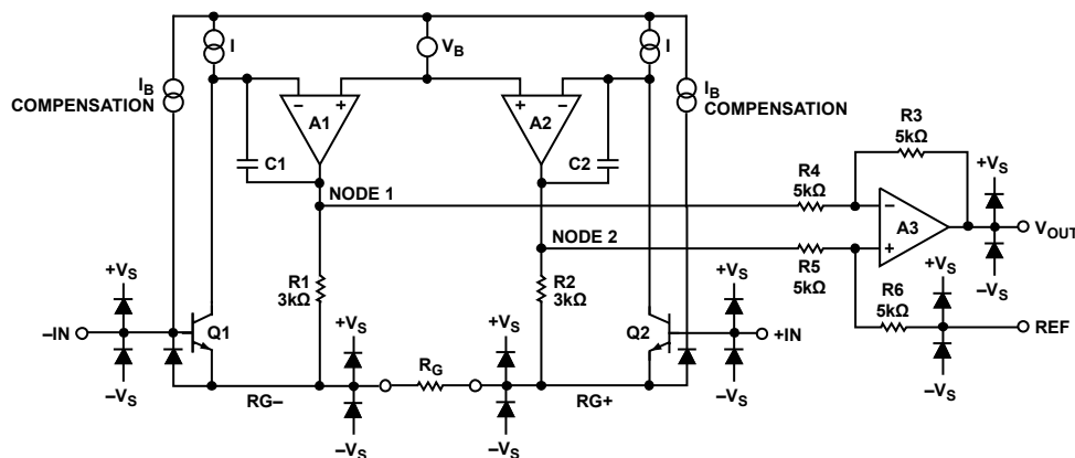
Figure 46. Simplified Schematic
