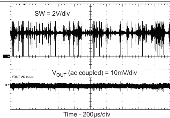
Figure 22. Pulse Skipping
