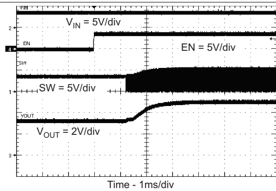
Figure 23. Start Up
