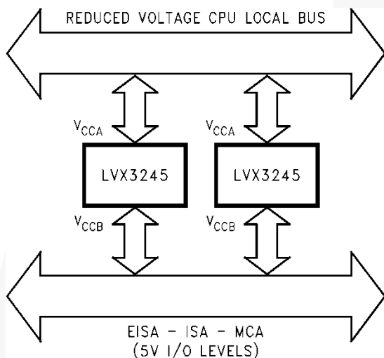
Figure 4. Application Example
