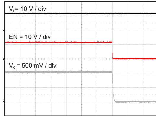
Time = 1 msec / div Figure 45. TPS563209 Shut Down Relative to EN
