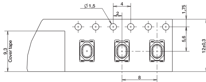
CARRIER TAPE
