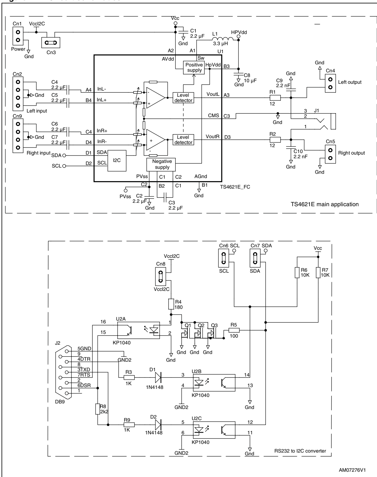
Figure 1. Circuit schematics
