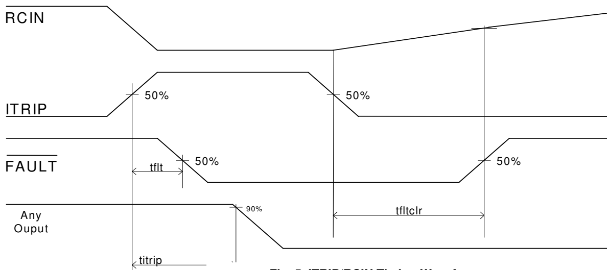
Fig. 5. ITRIP/RCIN Timing Waveforms
