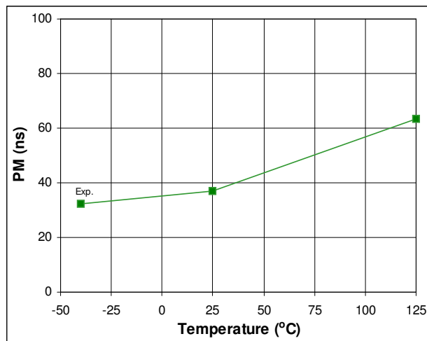
Fig. 15. Pulse Width Distortion vs. Temperature
