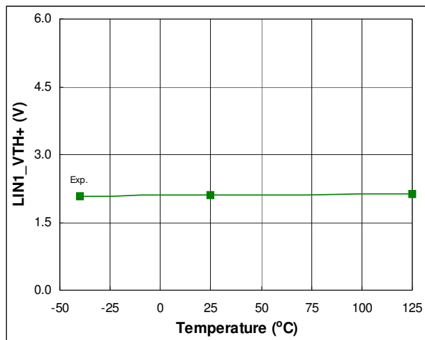
Fig. 21. Input Positive Going Threshold vs. Temperature
