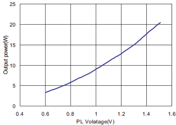
11. PL Voltage vs Output Power
