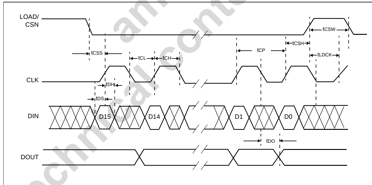
Figure 10. Interface Timing
