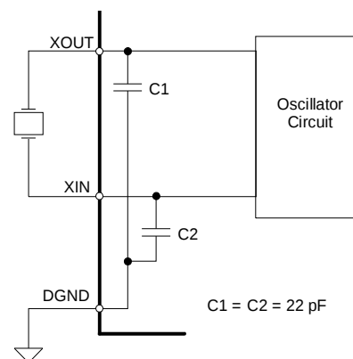
Figure 7. Oscillator Connections
