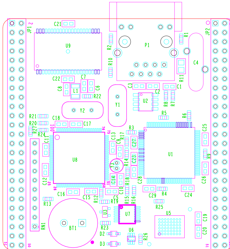
Figure 5. Top View
