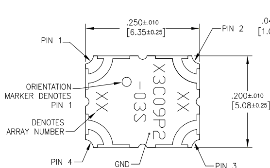
Dimensions are in Inches [Millimeters] X3C09P2-03S Mechanical Outline
